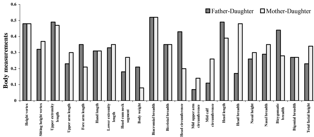
Figure 2. Parent-Offspring (PO) correlations in Body measurements
